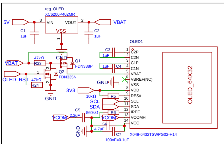
Ecran_OLED
